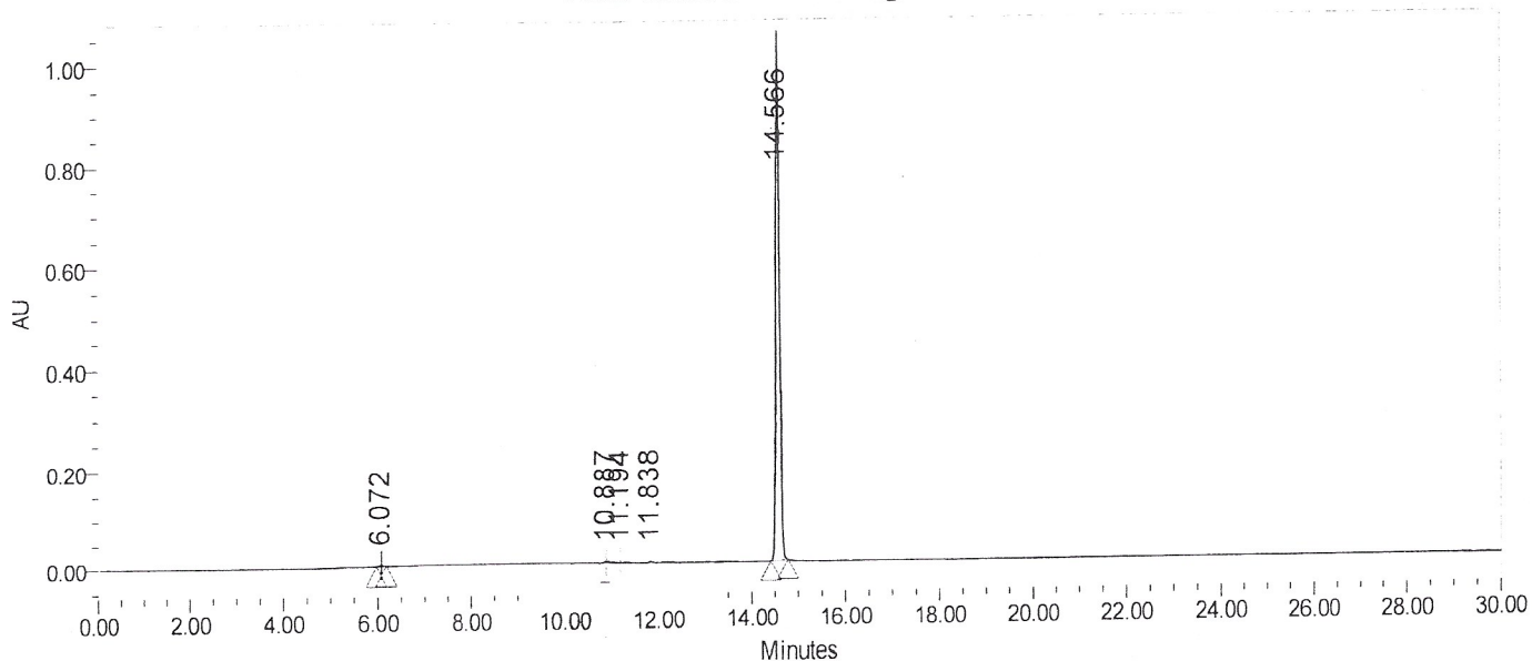
Auto-Scaled Chromatogram
